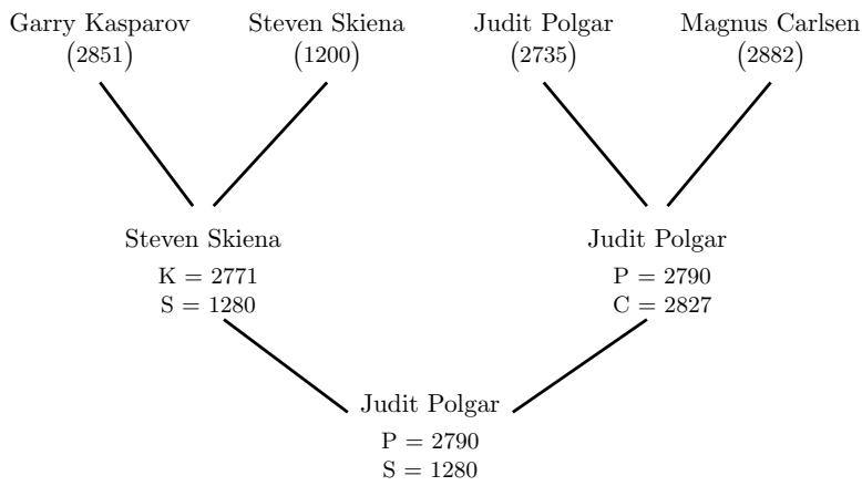
Figure 4.6: Changes in ELO scores as a consequence of an unlikely chess tournament.
