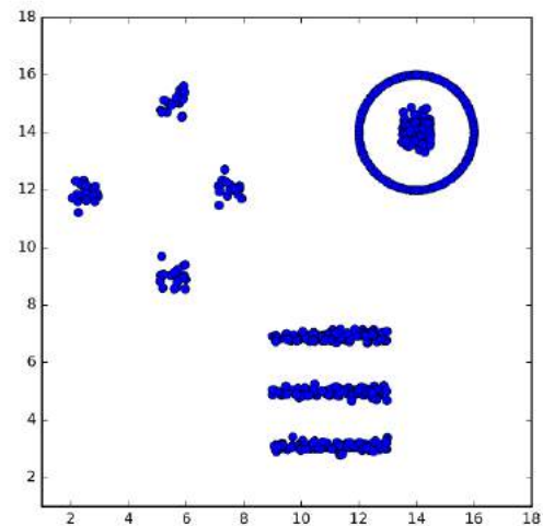
Figure 10.12: How many clusters do you see here?
